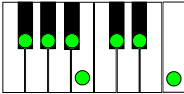
F# Major
