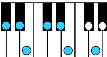
Db/C# Major
