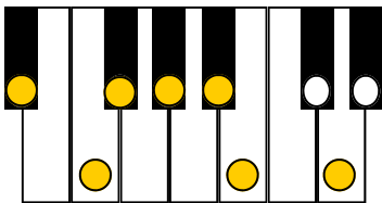
Ab/G# Major
