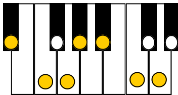
Eb Major
